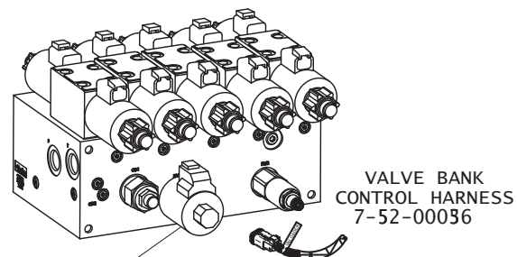
VIEW B-B
