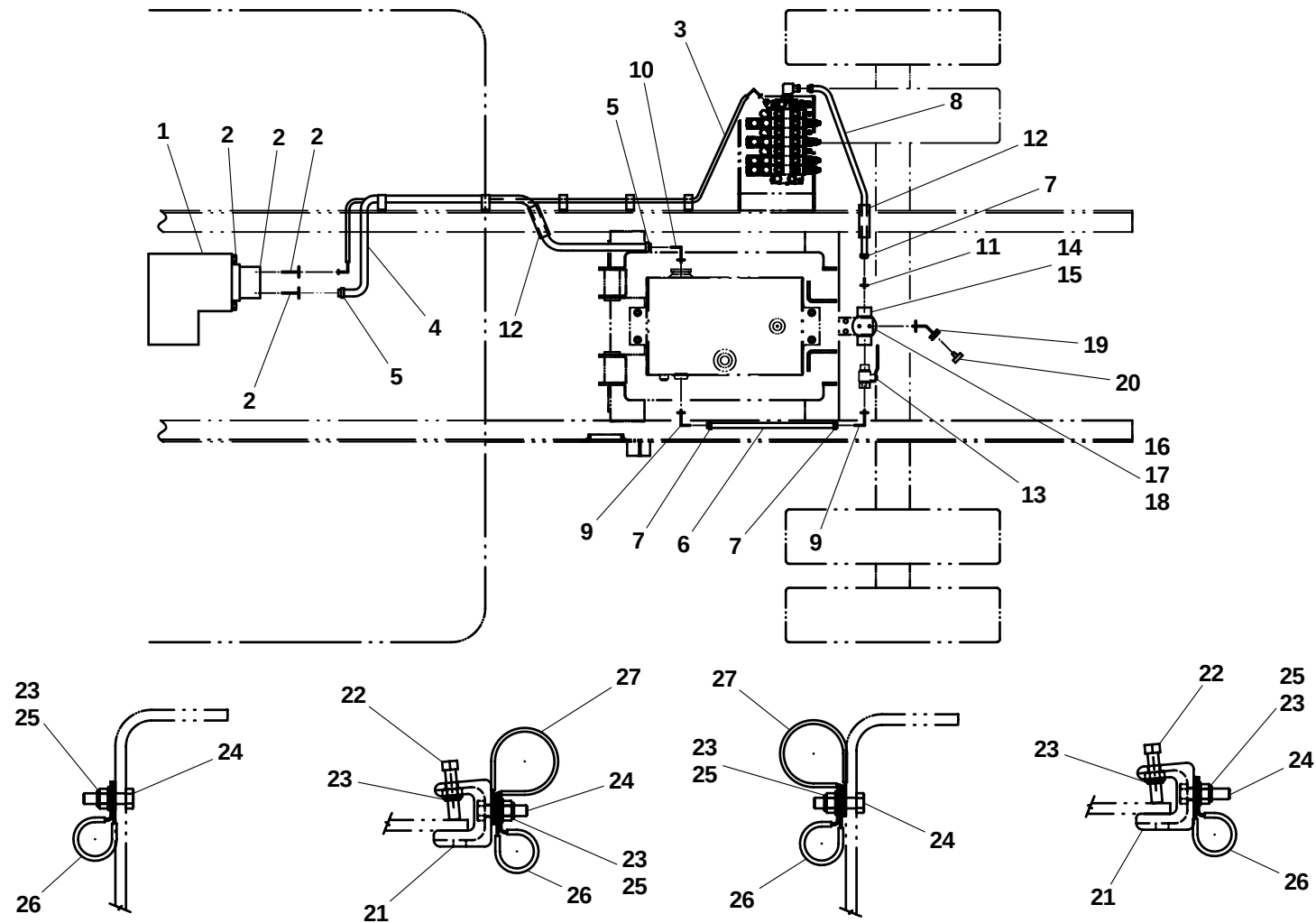
TYPICAL HOSE ROUTING / MOUNTING
